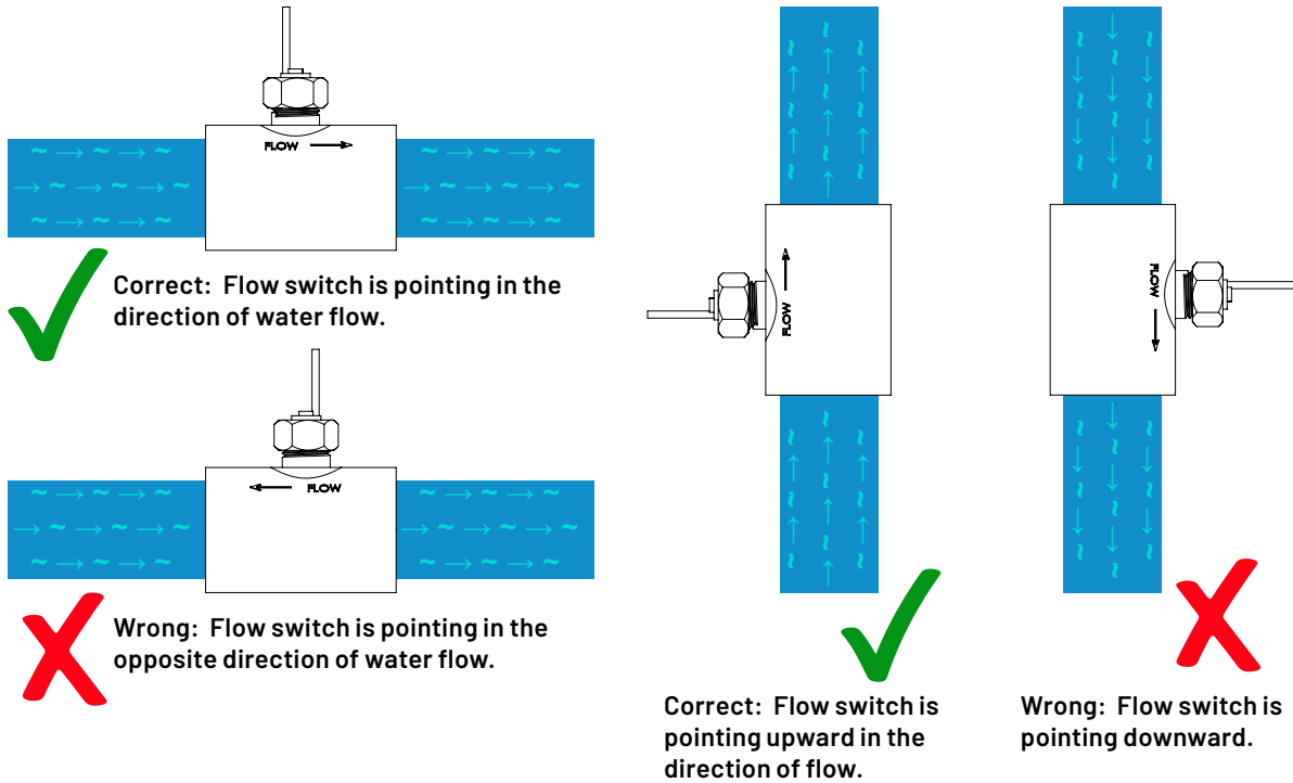
Figure 10. Flow switch orientation.
