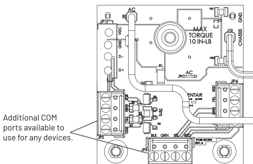
Figure 43: IntelliChlor SCG Circuit Board
