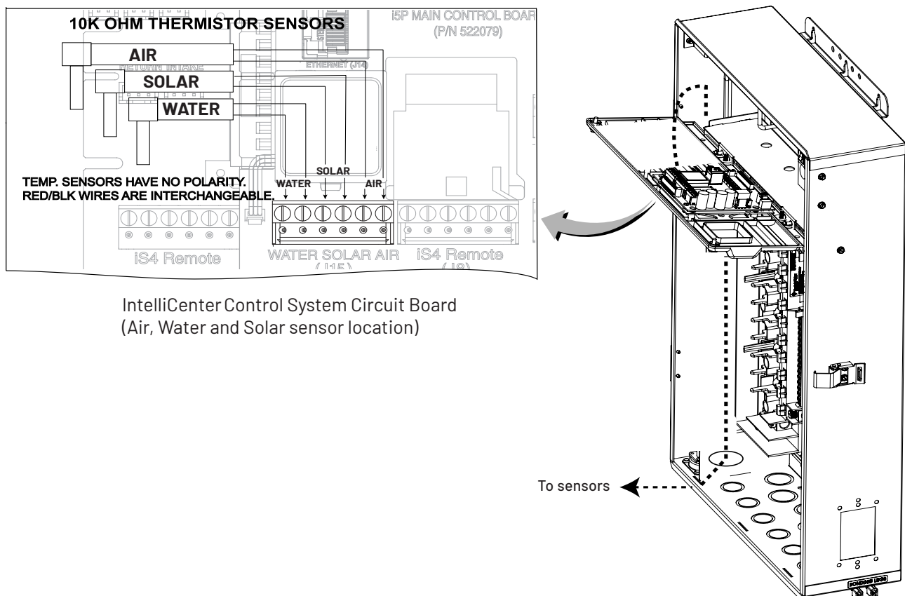
Figure 30: Location of temperature sensor terminals.
