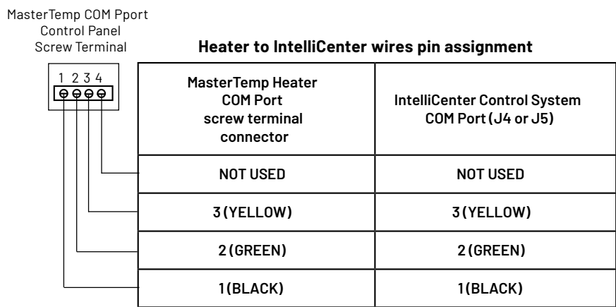
Figure 34: IntelliCenter COM Port connection for MasterTemp Heater
