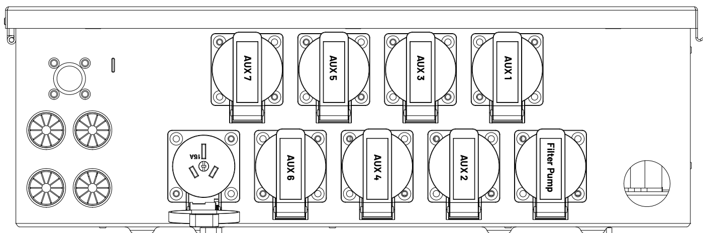
Figure 16: Electrical Outlets
