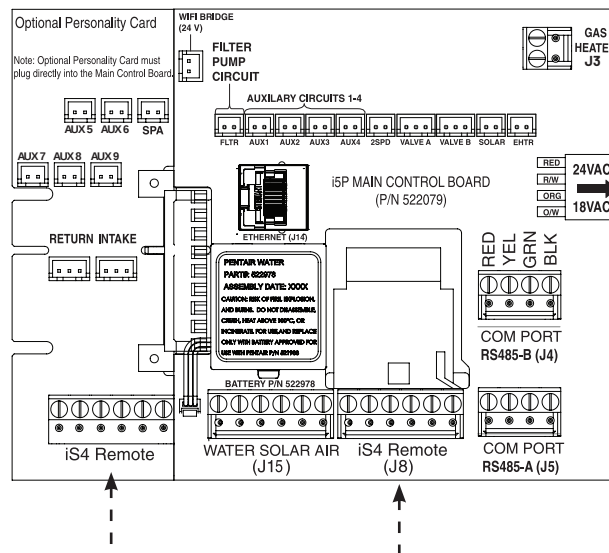
Figure 52: IntelliCenter iS4 Ports
