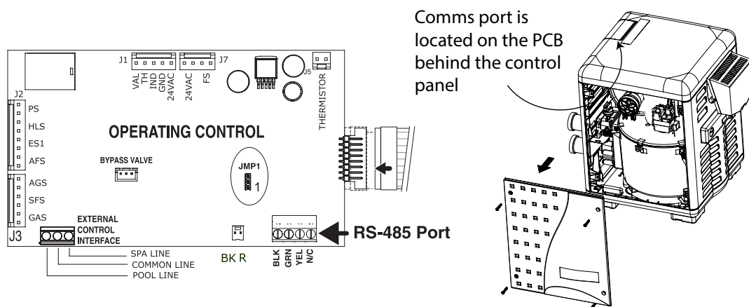
Figure 33: Location of MasterTemp COM Port.
