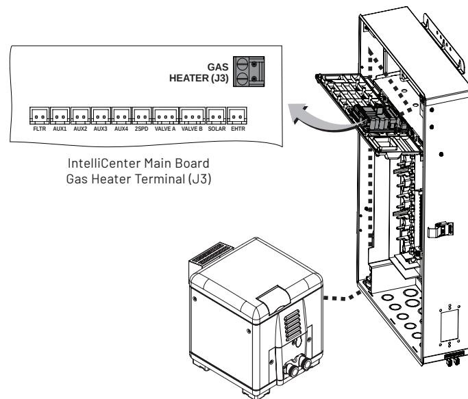
Figure 31: Location of gas heater terminal (J3) on IntelliCenter.
