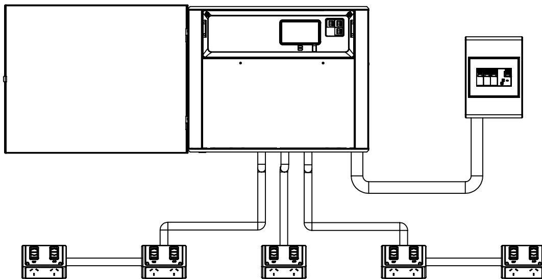
Figure 20: Electrical System Layout for Hard-Wired Unit with General Purpose Outlets
