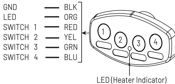
Figure 51: iS4 Spa Side Remote
