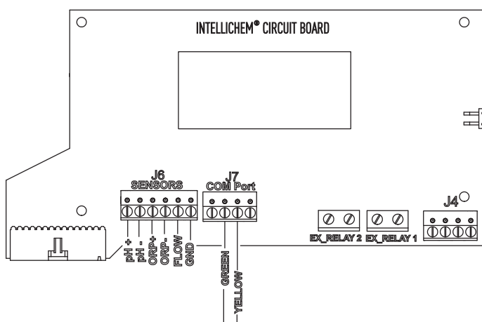
Figure 45: IntelliChem COMM port Connections.
