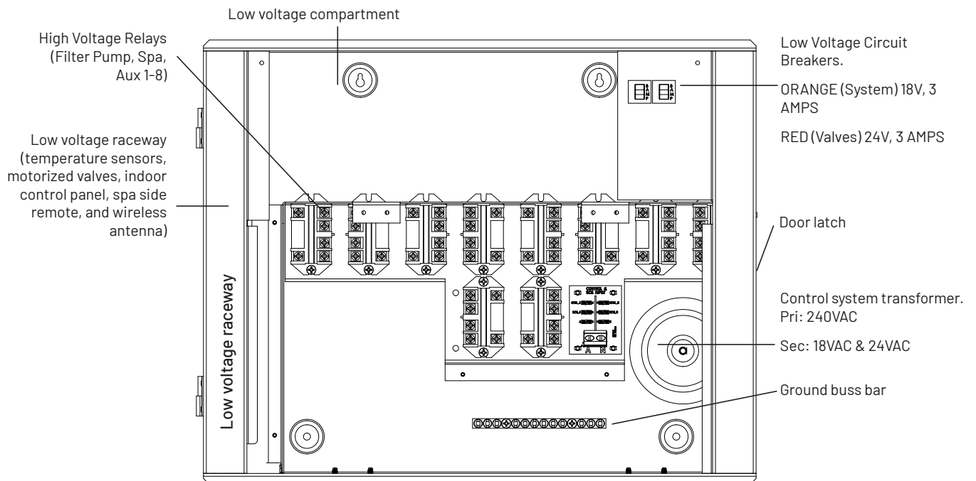
Figure 5: IntelliCenter i10D (Hard-Wired) view with control panel, door and HV cover panel removed.
