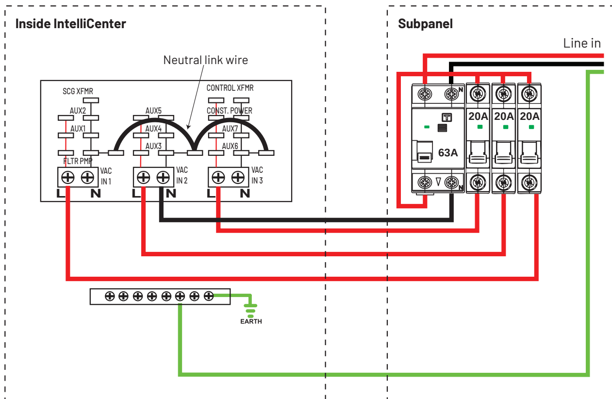
Figure 14: Electrical wiring using 1x 63A RCBO and 3x 20A CB's to supply IntelliCenter.
