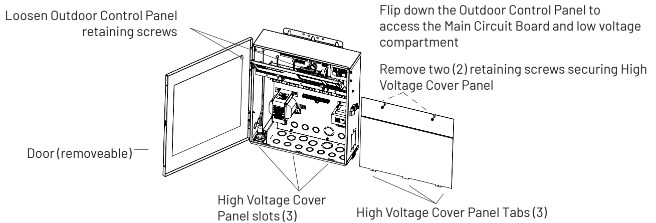
Figure 6: IntelliCenter power centre showing panels removed.
