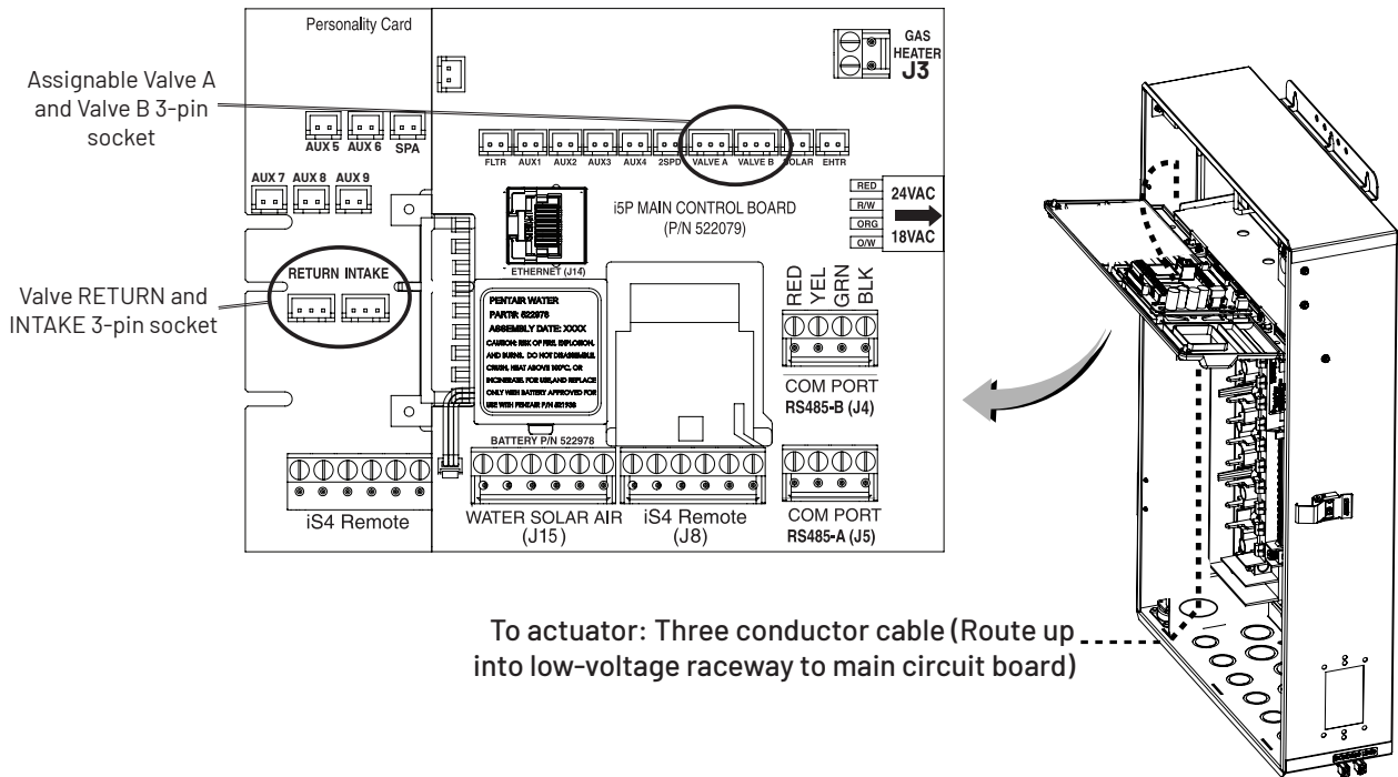
Figure 27: IntelliValve actuator mounting on a two-way valve.
