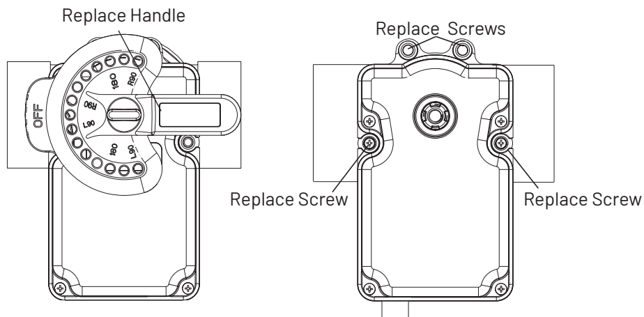
Figure 24: Actuator mounting screws. Use long screws provided with actuator.
