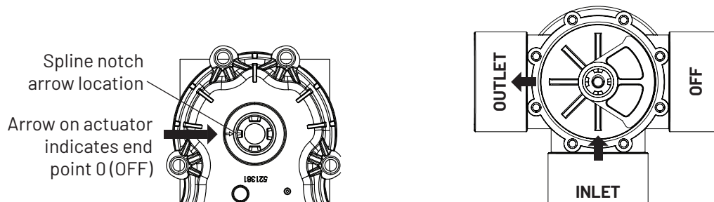
Figure 23: Actuator shaft spline (IntelliValve actuator shown).
