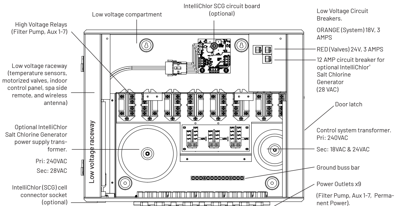
Figure 1: IntelliCenter PNP Power Centre view with control panel, door and HV cover panel removed.
