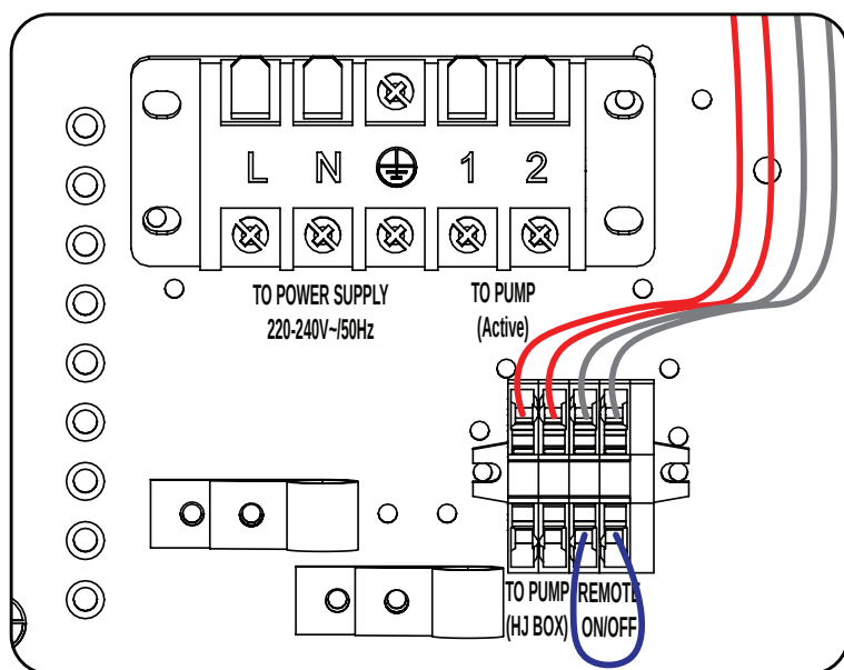
Figure 35: Control Port connection for UltraTemp Hxi Heat Pump
