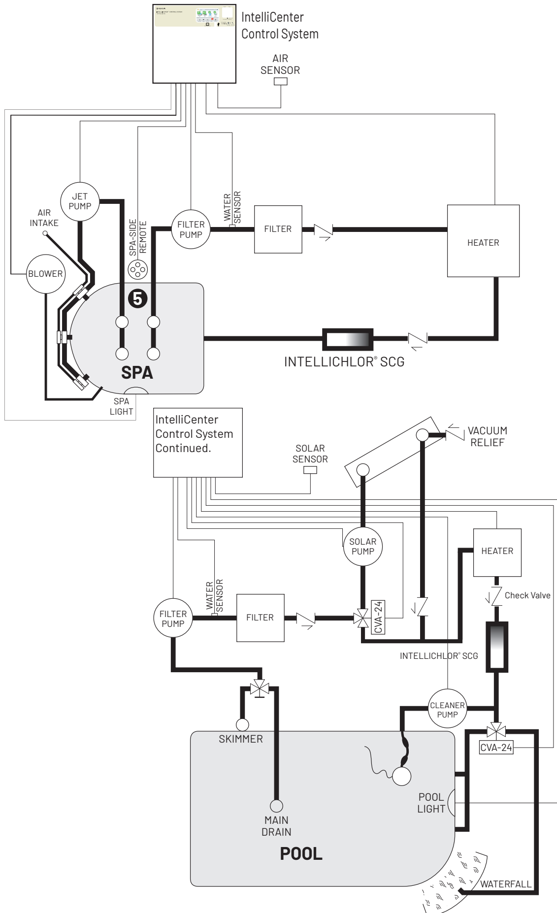
Figure 61: IntelliCenter Plumbing Layout for Seperate Pool/Spa
