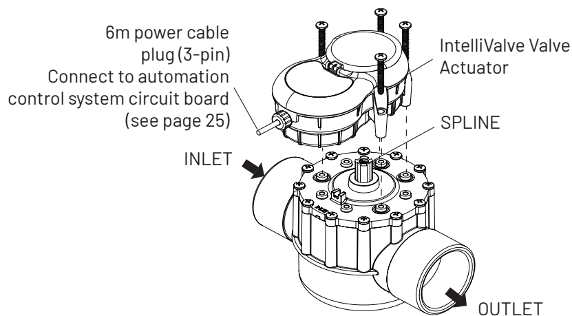
Figure 26: IntelliValve actuator mounting on a two-way valve.
