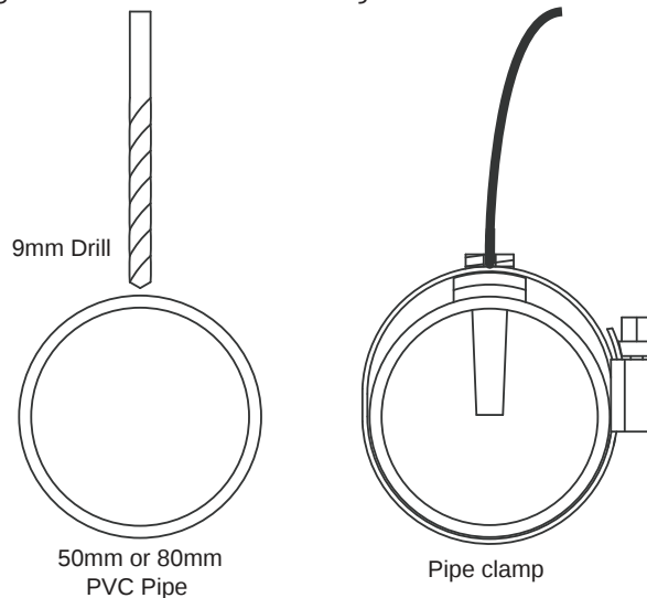
Figure 29: Cross section view of water temperature sensor installation.
