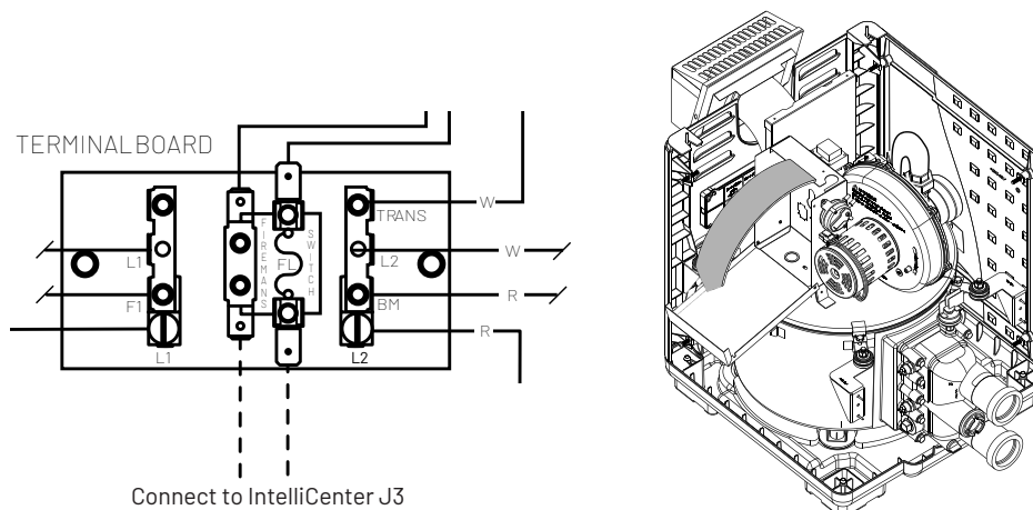
Figure 32: Location of MasterTemp FiremanSwitch terminals.
