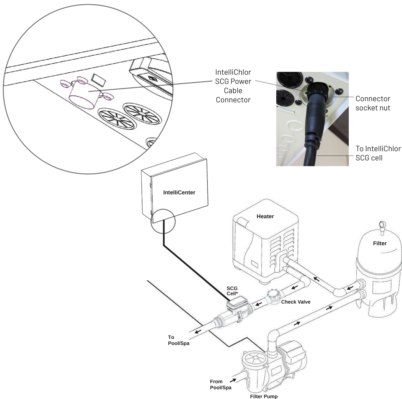
Figure 41: IntelliChlor COM Port location.
