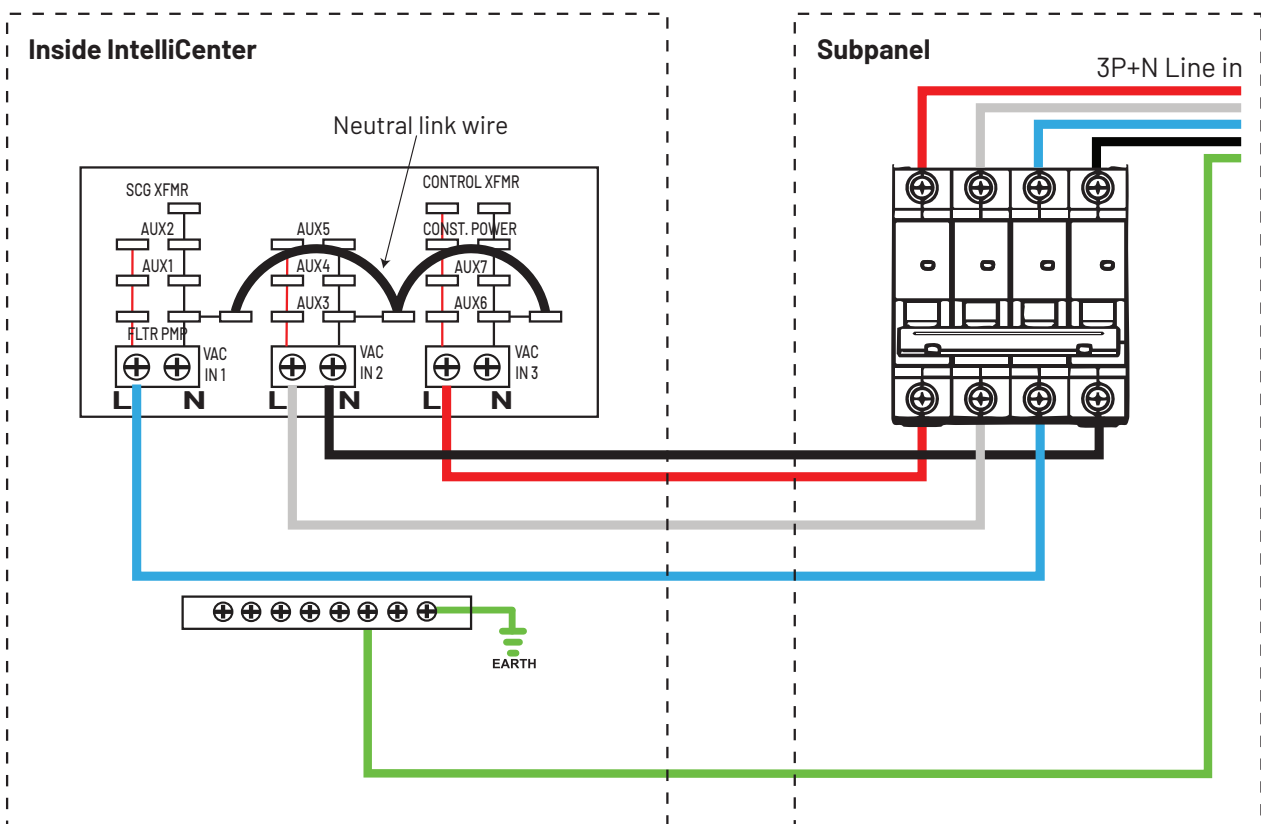
Figure 15: Electrical wiring using a 3-Phase, 4-Pole RCBO to supply IntelliCenter.
