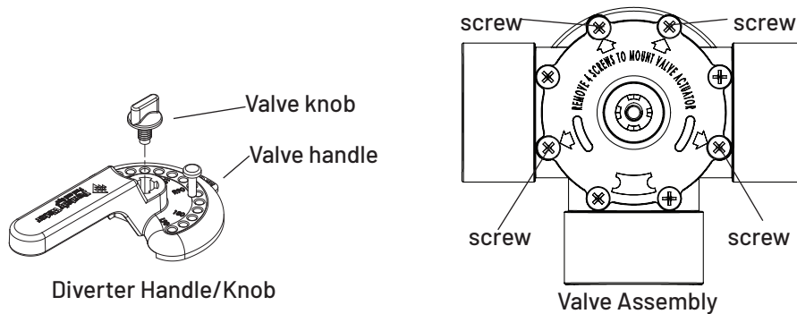
Figure 22: Actuator mounting screws on Pentair 3-way valve.
