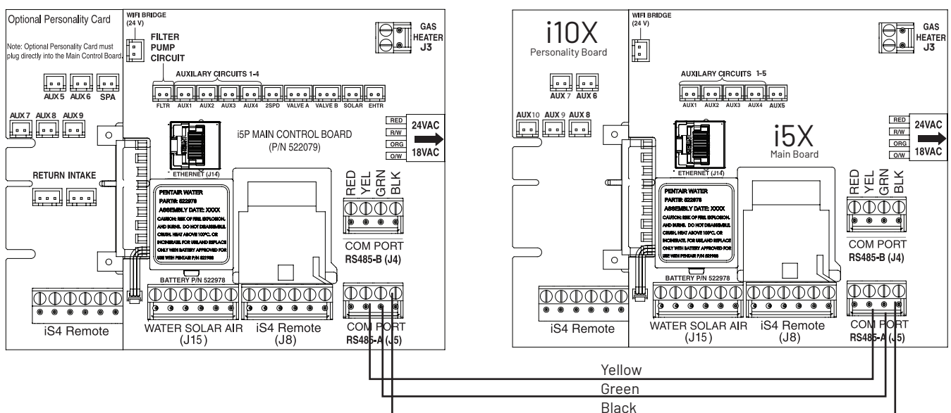
Figure 57: Expansion Center COMM Port Connection.
