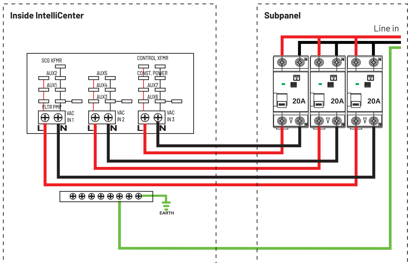
Figure 13: Electrical wiring using 3x 20A RCBO's to supply IntelliCenter.
