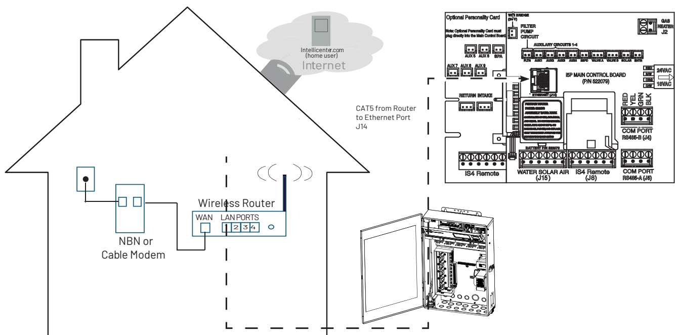
Figure53: IntelliCenter Ethernet Connection.
