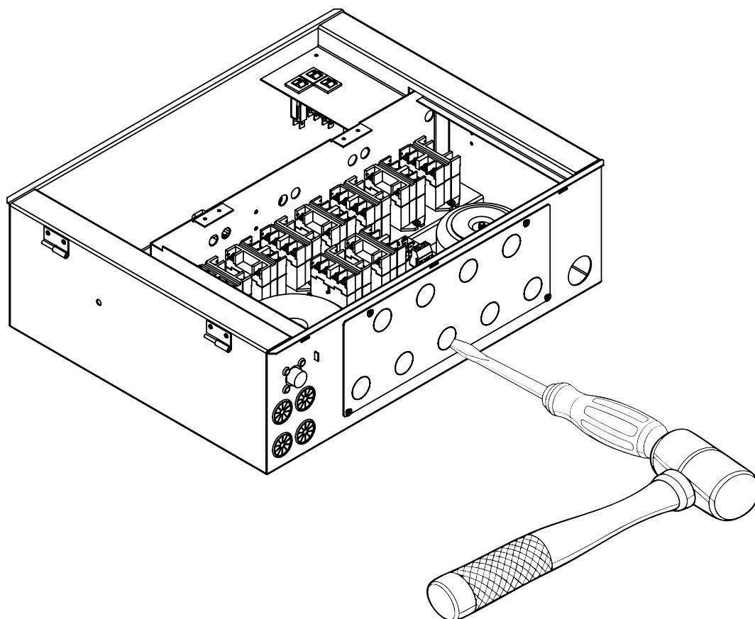
Figure 19: Location and method for making conduit holes in hard-wired units.
