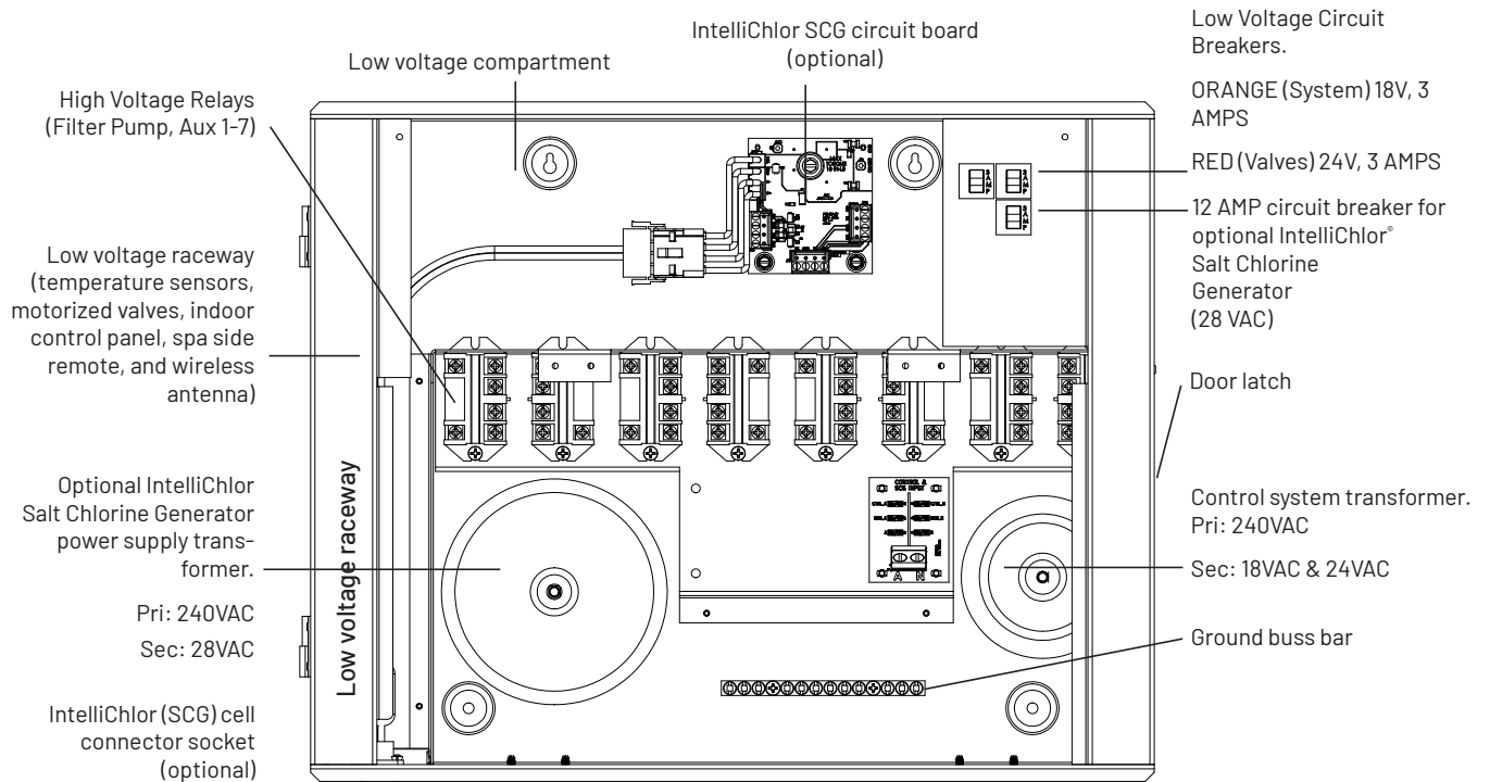
Figure 4: IntelliCenter i8PS (Hard-Wired) View with control panel, door and HV cover panel removed.
