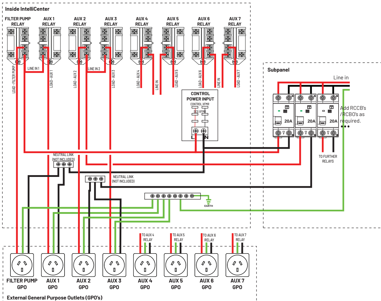
Figure 18: Electrical wiring using 3x 20A RCBO's to supply IntelliCenter.
