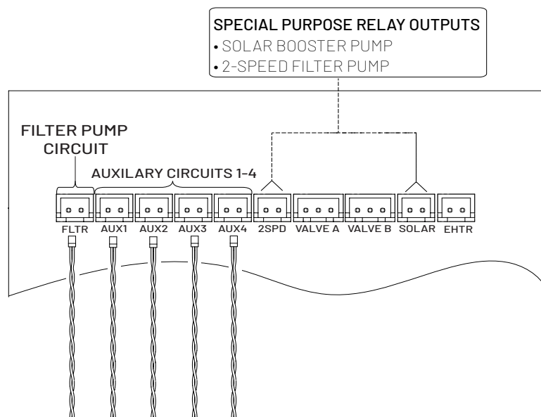
Figure 21: Relay coil wires to IntelliCenter main board.
