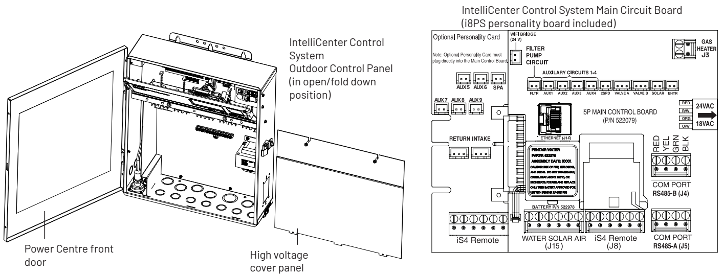
Figure 2: IntelliCenter power centre view with control panel down revealing main board.
