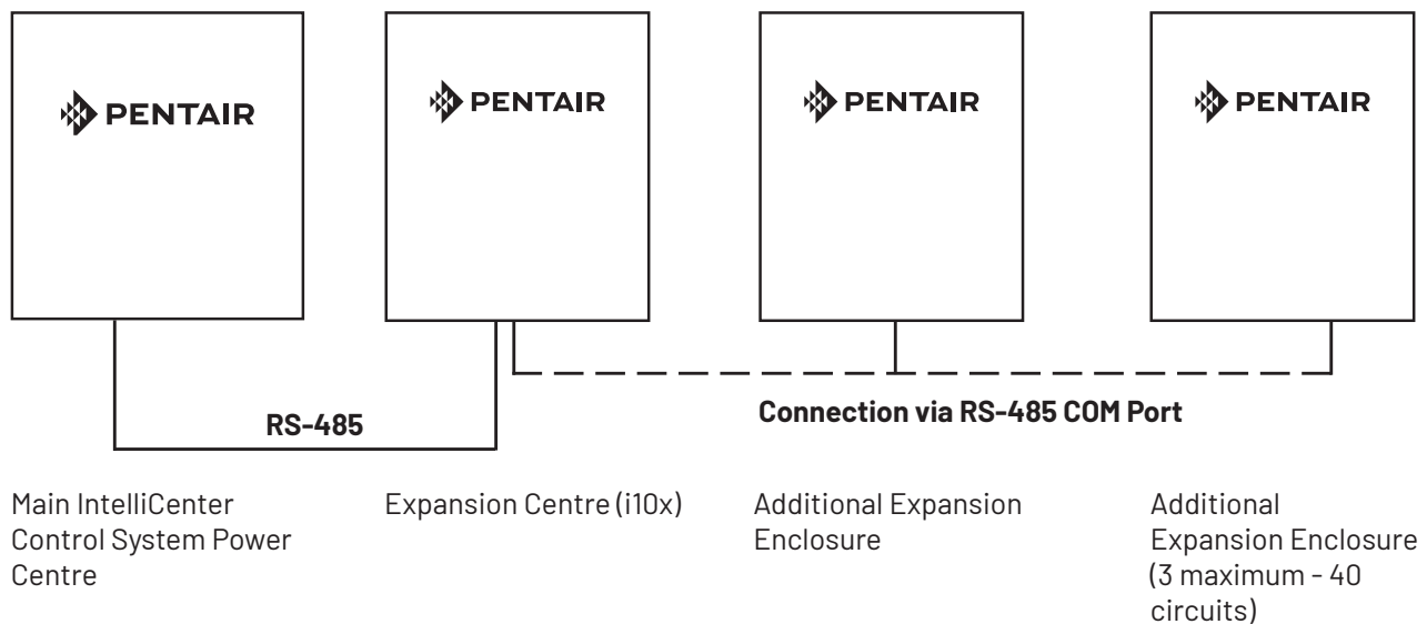
Figure 56: Expansion Center Layout
