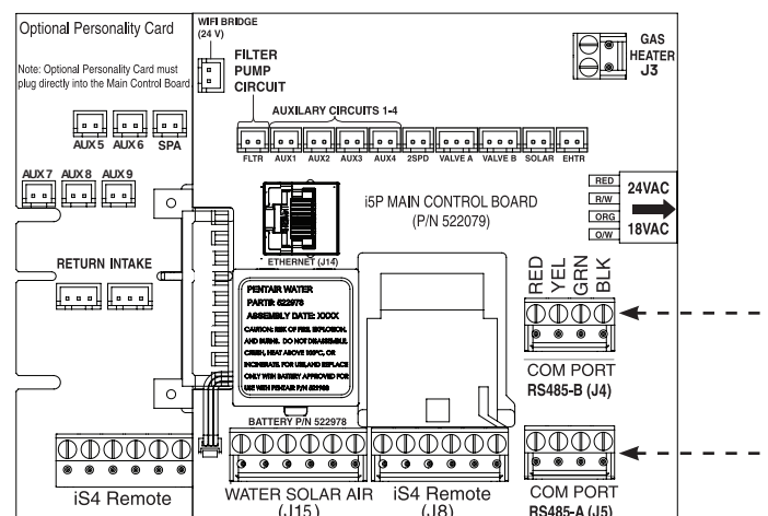
Figure 48: IntelliCenter COM Ports
