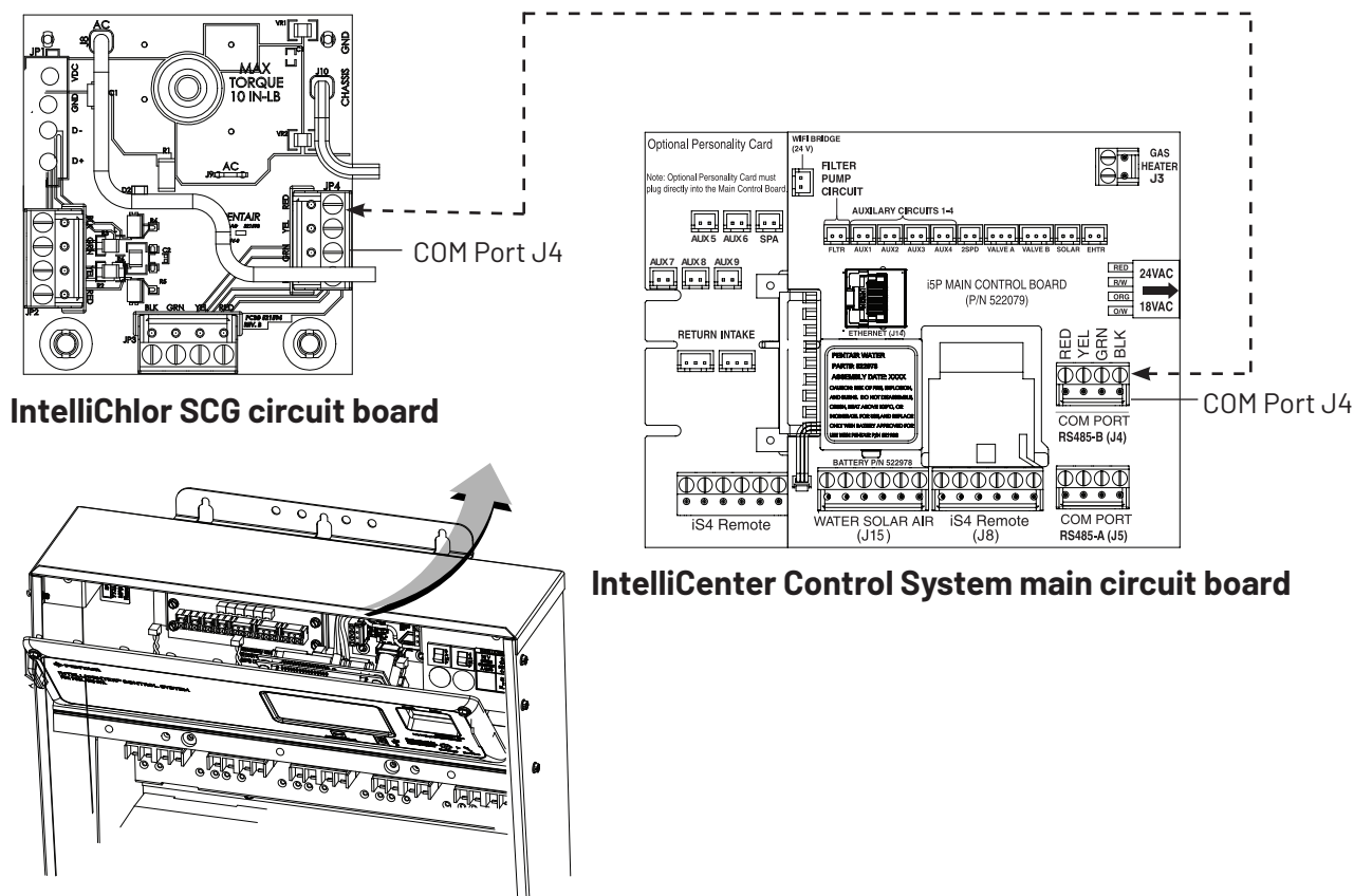
Figure 42: IntelliCenter Control System (with IntelliChlor SCG option)
