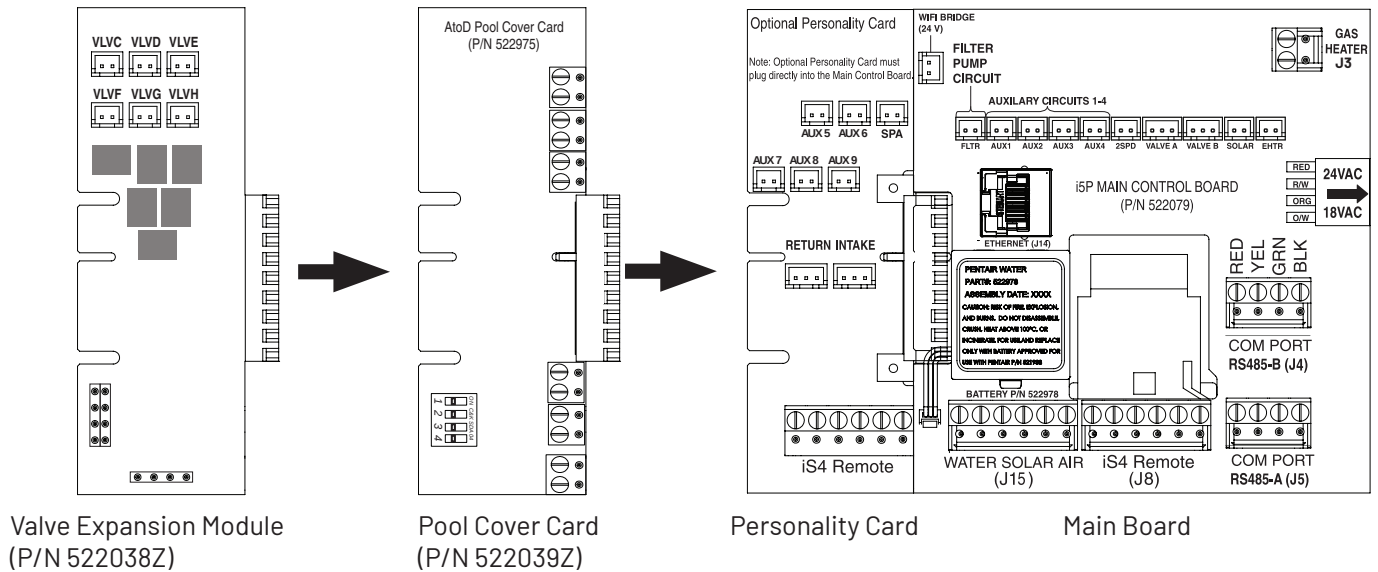
Figure 54: Expansion Card Installation on Main Board
