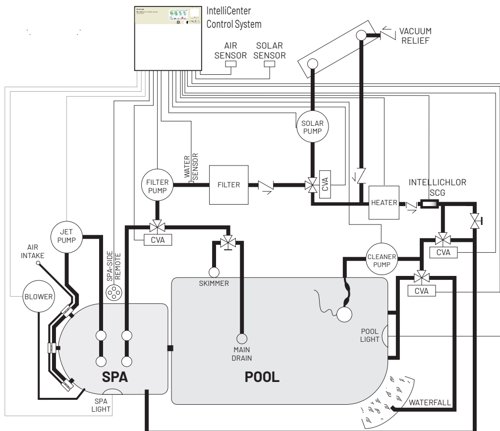
Figure 60: IntelliCenter Plumbing Layout for Pool/Spa
