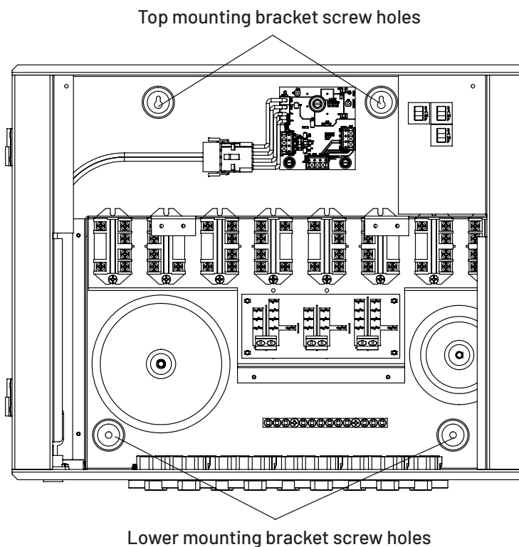
Figure 7: IntelliCenter power centre mounting holes.
