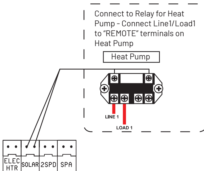
Figure 36: IntelliCenter Heat Pump Relay for Heat Pump and Gas Heat combination
