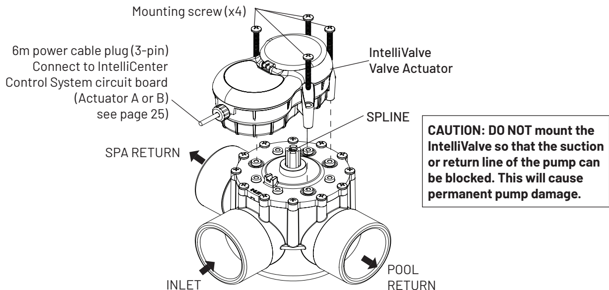
Figure 25: IntelliValve actuator mounting on a three-way valve.
