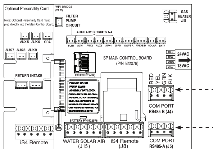
Figure 44: IntelliCenter COMM port locations.
