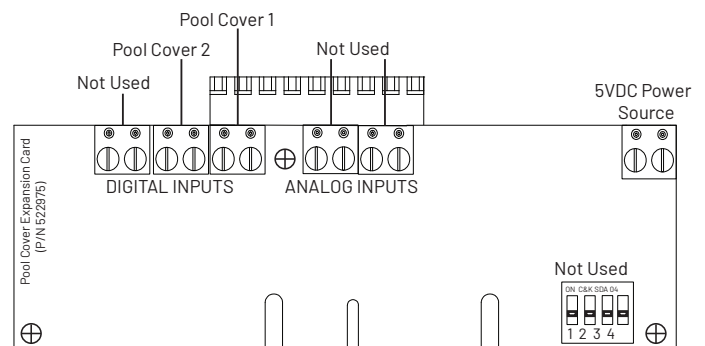
Figure 55: Pool Cover Expansion Card
