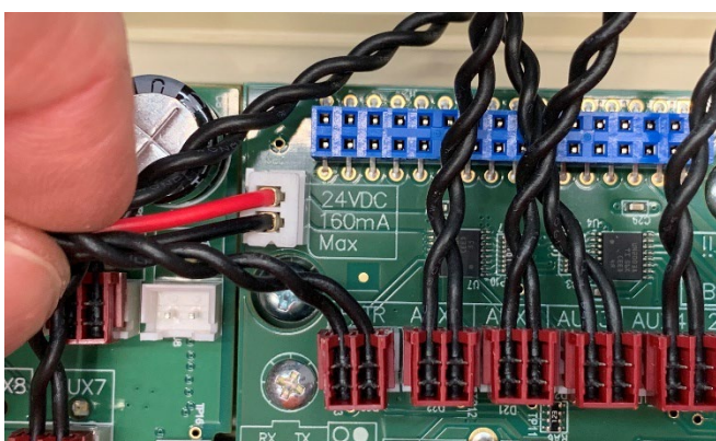
Step 9 – Connect the power cable to the IntelliCenter main board, terminal is marked 24VDC.
