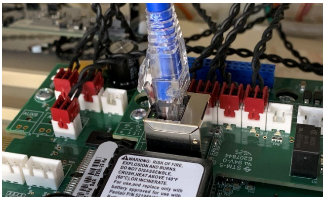
Step 7 – Connect the ethernet cable to the IntelliCenter main board.
