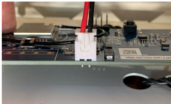
Step 10 – Connect the power cable to the wifi board. Close the IntelliCenter control panel and secure the two screws. Switch on power to the IntelliCenter at the breaker.
